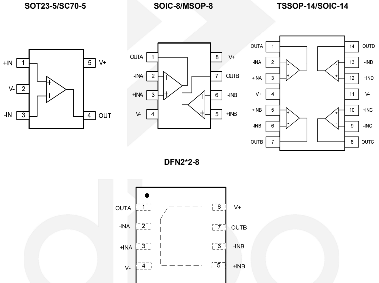
Figure 1 Pin Assignment
