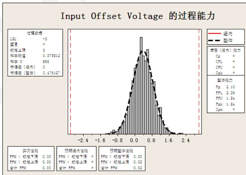
Input Offset Voltage Statistics
